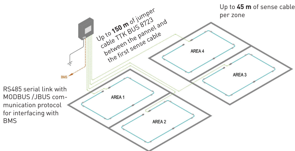
Figure 1.2.4 : Layout of FG-ALS4 with 4 zones
