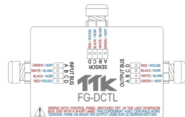
Figure 1.4.4.1: Interface box FG-DCTL cabling diagram
