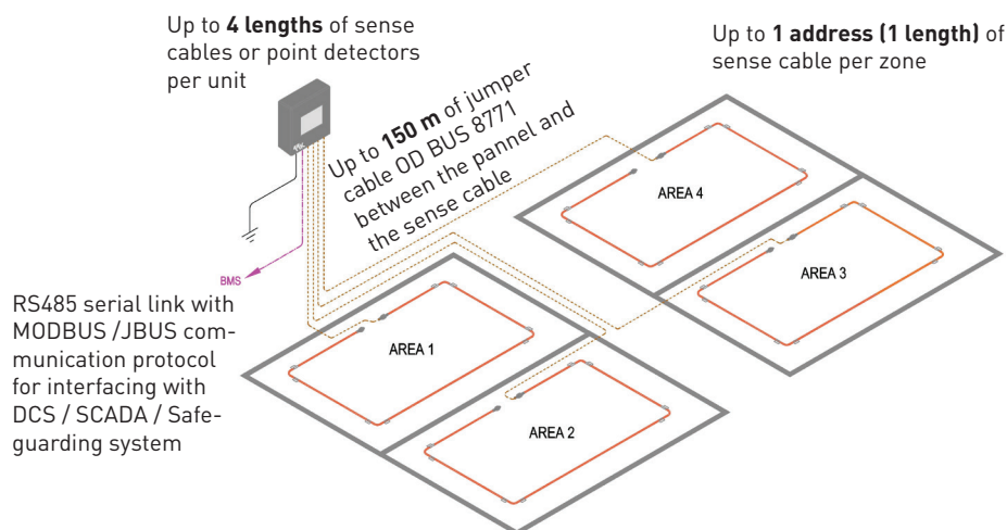
Figure 1.2.5 : Layout of FG-ALS4-OD with 4 zones
