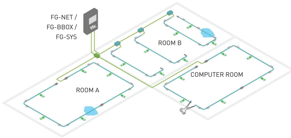
Figure 1.4.3 : Layout with FG-DTC et FG-DTCS boxes
