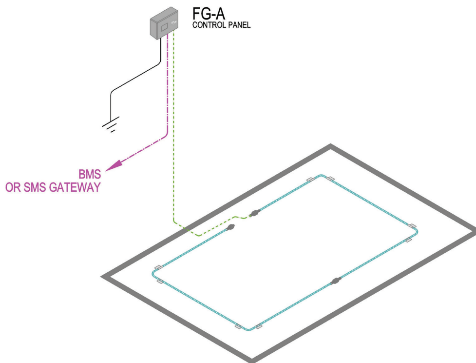
Figure 1.2.6 Layout with FG-A
