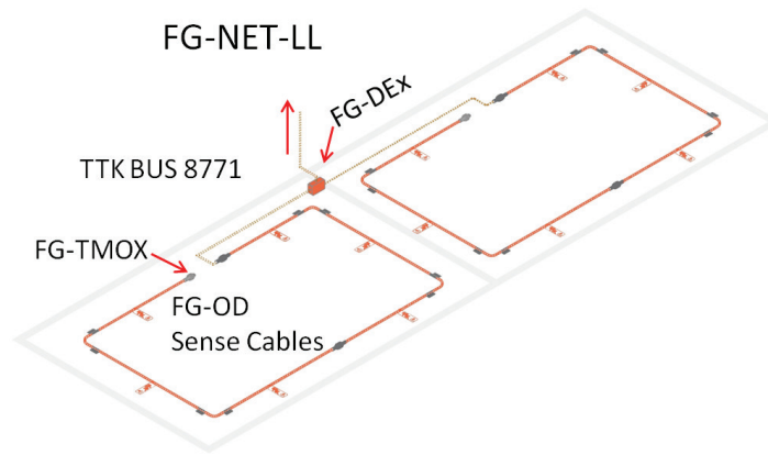
Figure 1.4.8 : Layout of diversion box FG-DEx
