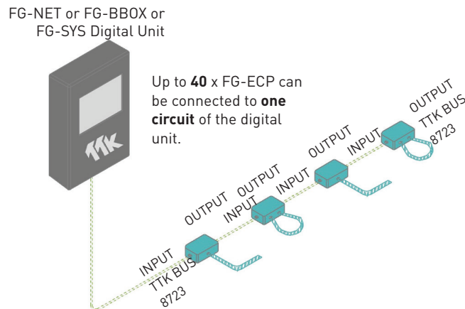
Figure 1.3.1: Layout of FG-ECP with FG-NET
