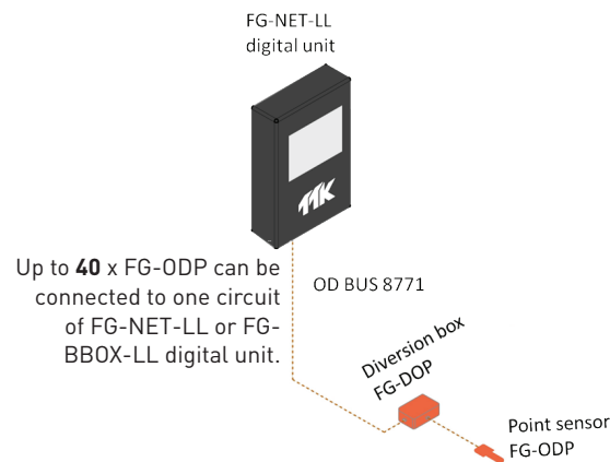
Figure 1.3.2: Layout of point sensor FG-ODP with FG-NET-LL digital unit using FG-DOP box
